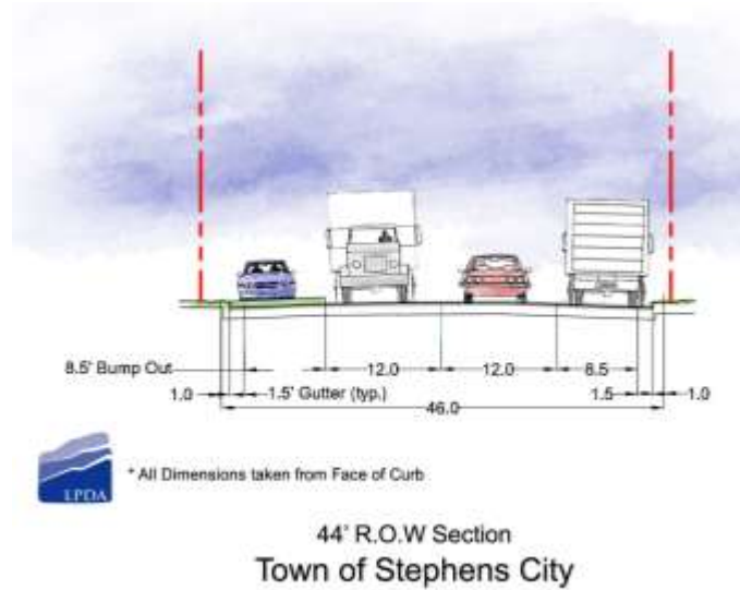
Figure 5- 44 Foot Cross Section.
