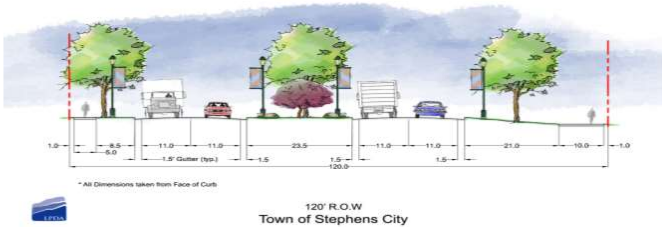
Figure 3- 120 Foot Cross Section.
