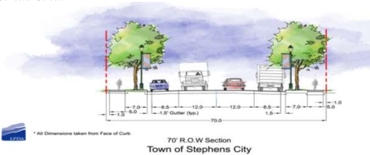
Figure 4- 70 Foot Cross Section.
